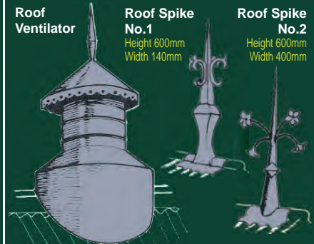
Small - Height 980mm min. diameter - 200mm Base diameter 360mm
